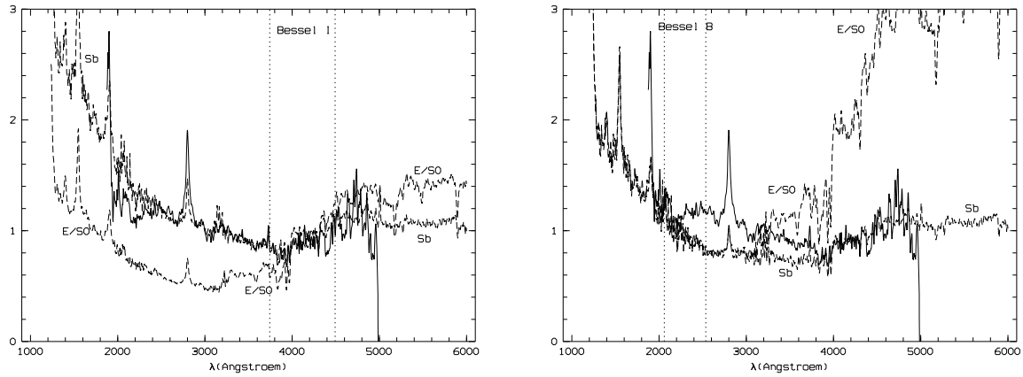
Fig. 4. Simulation of the spectrum of FDF0809 in the I -band (left) and B -band (right). The solid line shows the measured spectrum in the restframe, the dashed lines show the simulated spectra (QSO+galaxy spectra added up) marked with the model type of the galaxy template. The wavelength range used for scaling is marked with dotted lines and the name of the corresponding filter. The Sb-model is unambiguously preferred in both cases.
